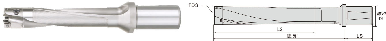
EMDG 5D Force drill connecting rod
