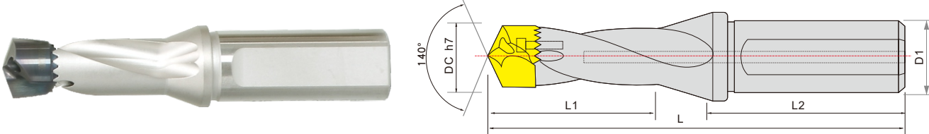
■ SMD 8D Multi purpose crown bit
