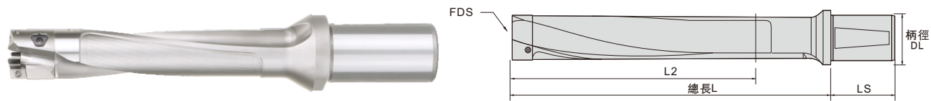
EMDG 1.5D Force drill connecting rod
