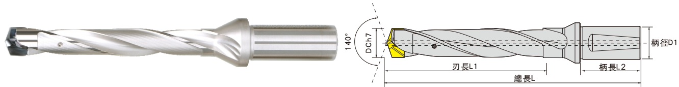
EMD-3D Rear locking crown drill bit
