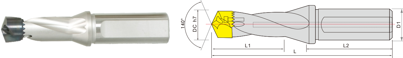
■ SMD 10D Multi purpose crown bit
