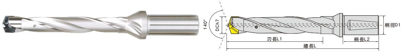
EMD-8.5D Rear locking crown drill bit
