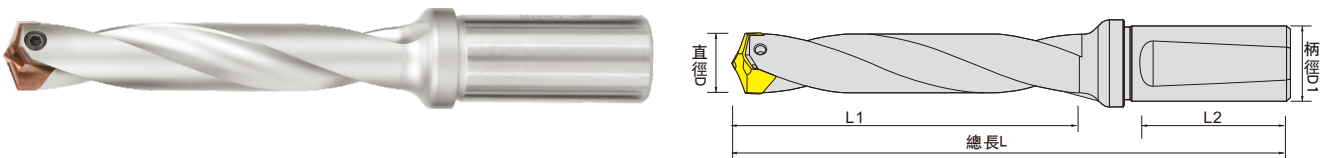
■ SDT 7D Side lock type Crown drill bit
