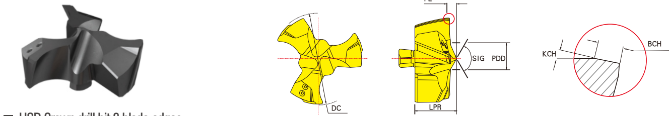
■ HSD Crown drill bit 3 blade edges
