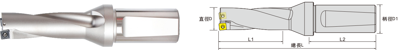
■ SP-4 Fast C20 drilling
