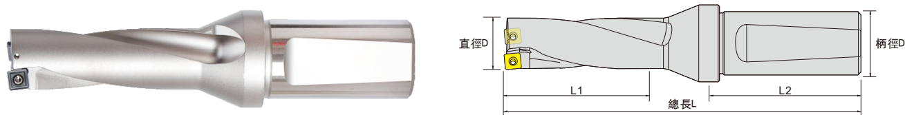
■ SP-3 Fast drilling
